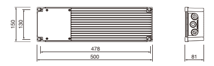
智能一体式驱动 Intelligent driver
